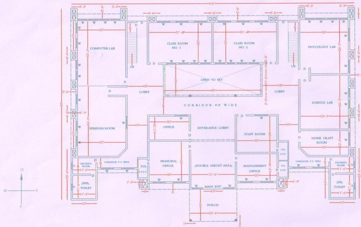
GROUND FLOOR PLAN { COVD. AREA = 12263 SQ.FT. OR 1139.68 SQ.MT.
