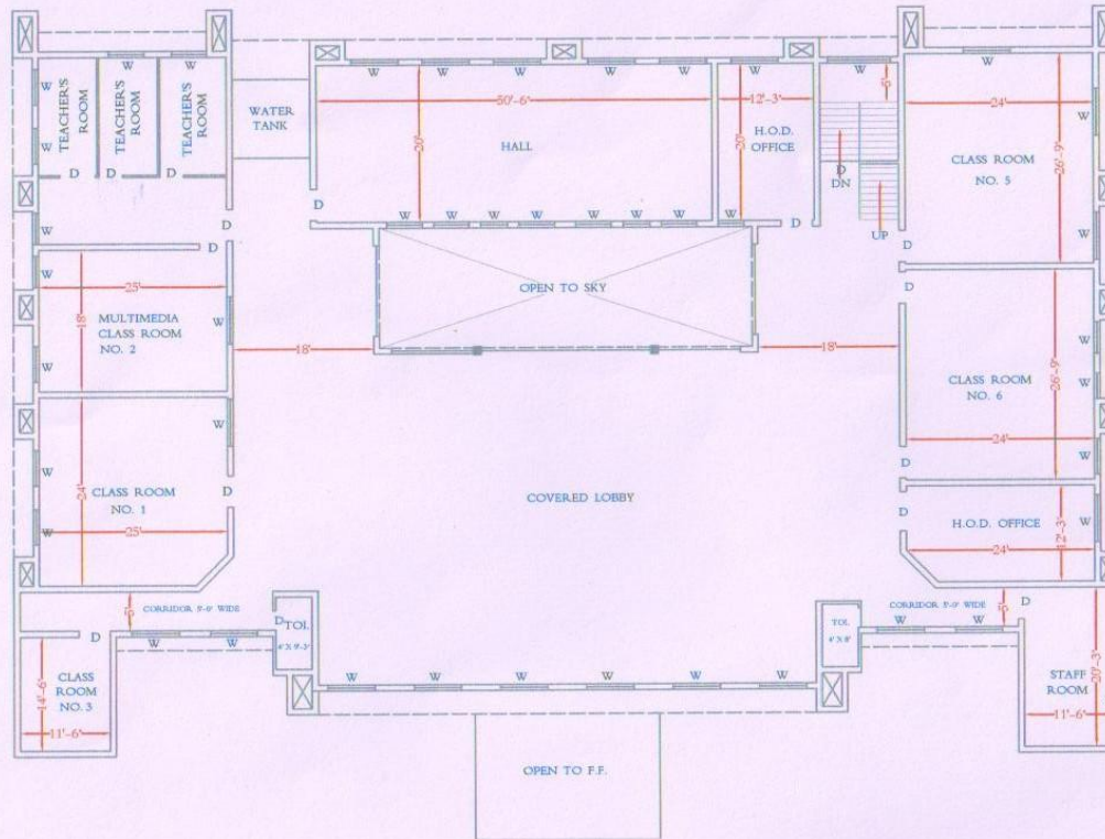
SECOND FLOOR PLAN { COVD. AREA - 11888 SQ.FT. OR 1104.83 SQ.MT.
