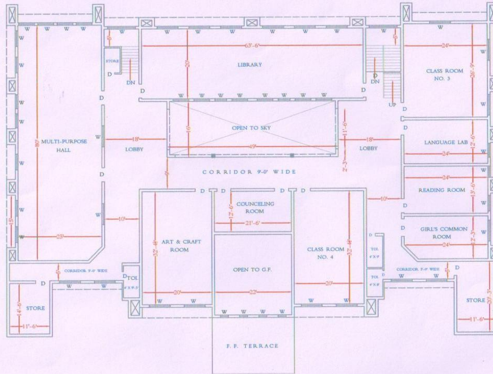
FIRST FLOOR PLAN { COVD. AREA = 11888 SQ.FT. OR 1104.83 SQ.MT.
